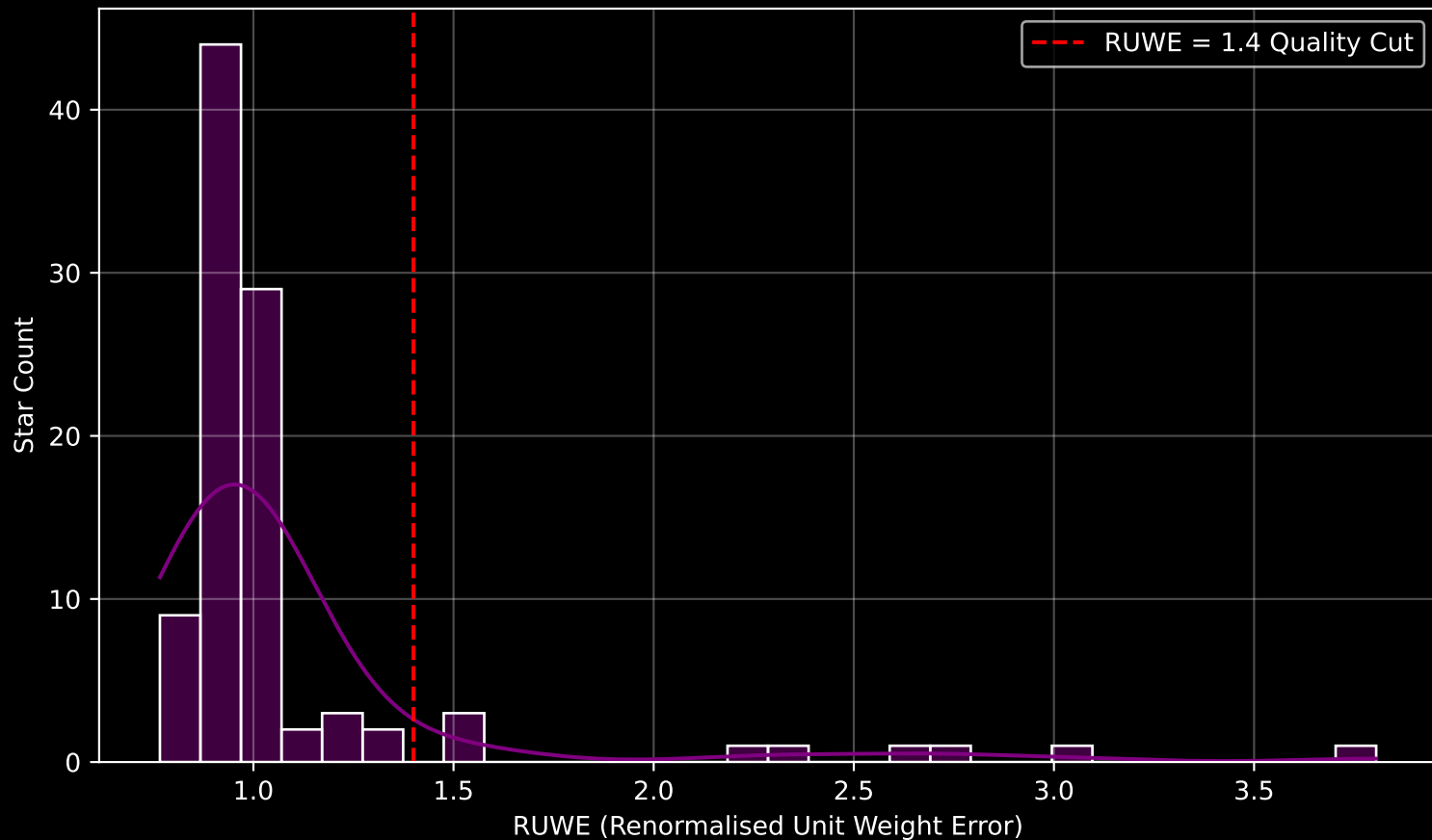
GAPOGEE DR17 Field [007+07] RUWE Distribution (n= 98)
