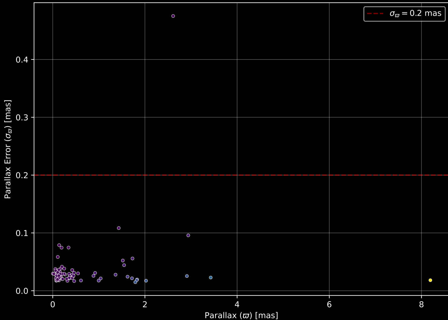
APOGEE DR17 Field: [007+07] Parallax Quality (n= 99)
