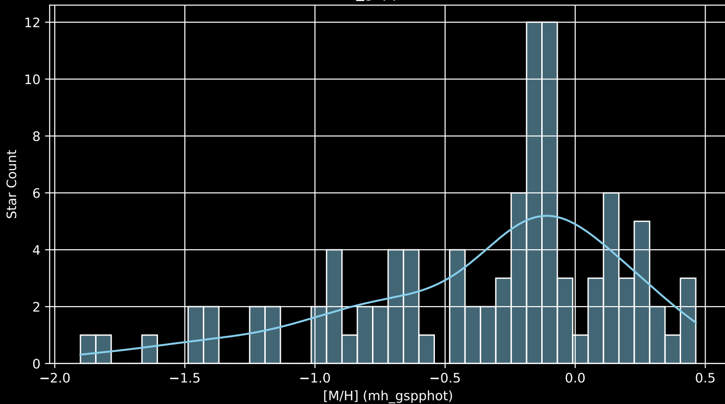
APOGEE DR17 Field: [007+07] [M/H] (mh_gspphot) (n= 99)
