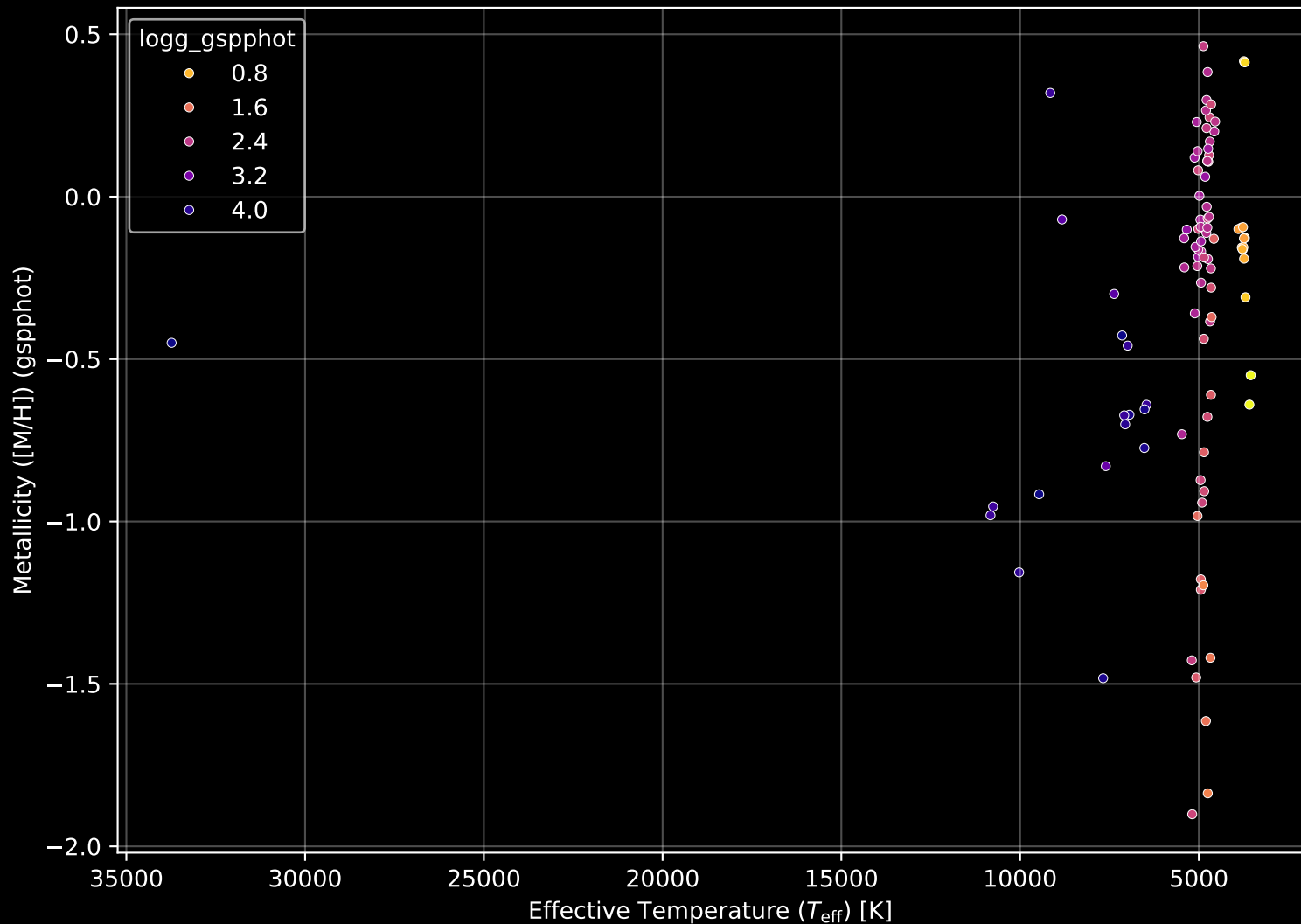
APOGEE DR17 Field: [007+07] Stellar Population Parameters (n= 99)
