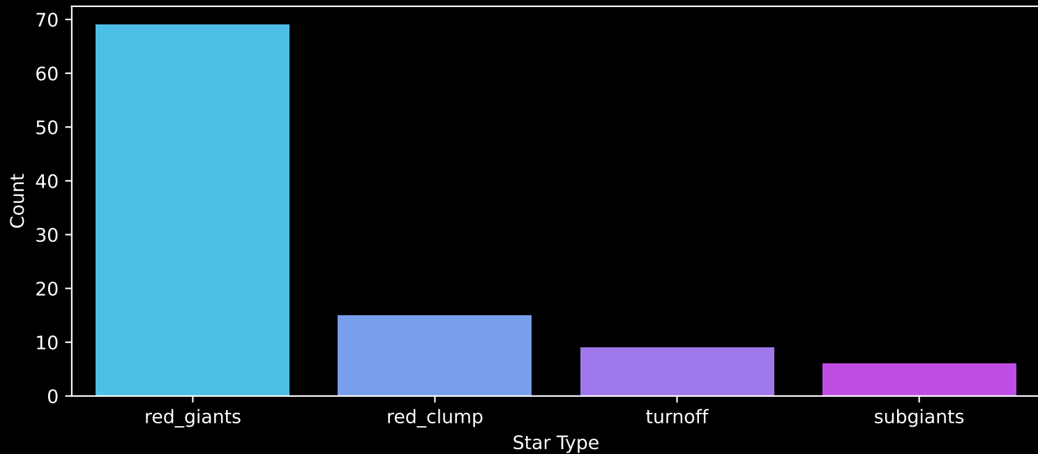
APOGEE DR17 Field: [007+07] Count plot of Star Type
