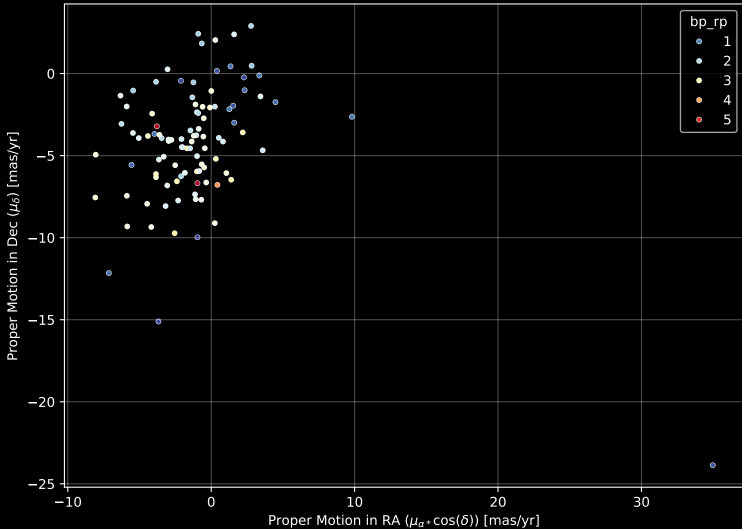
APOGEE DR17 Field: [007+07] Proper Motion Diagram (n= 99)
