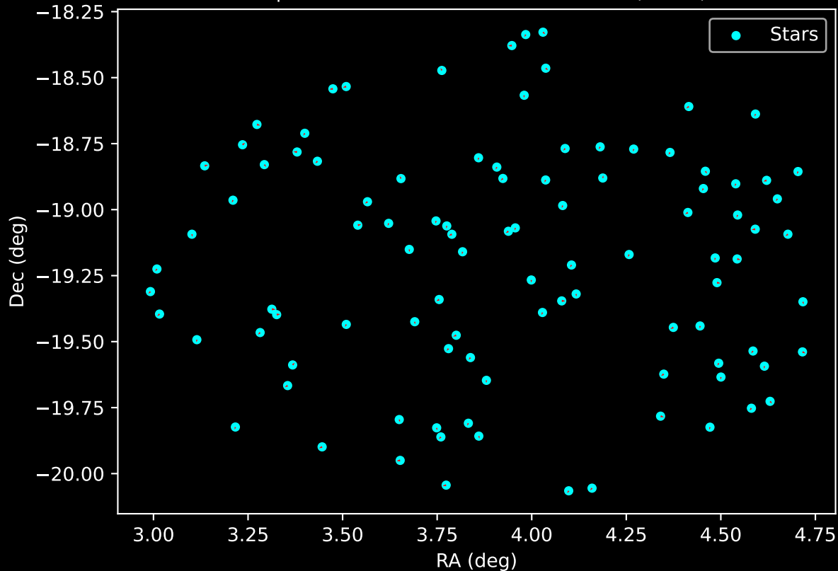
APOGEE DR17 Field: [007+07] Proper Motion Vectors for Gaia Star Field (n= 99)
